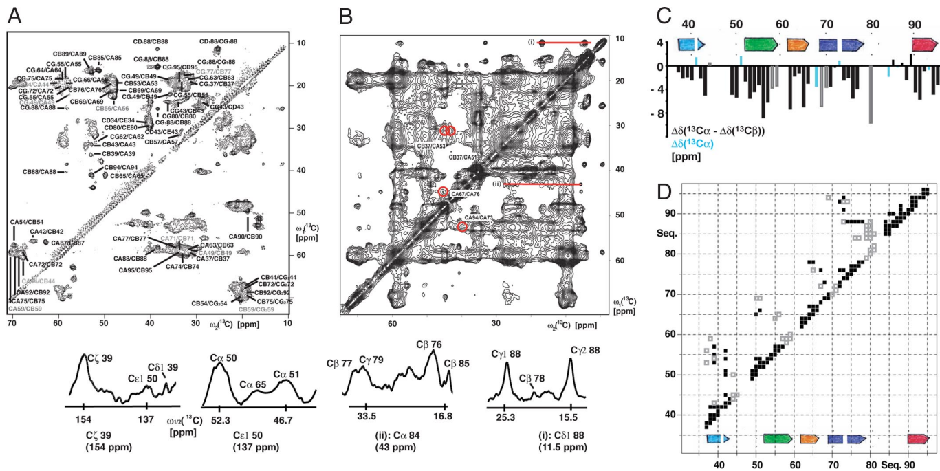
Fig. 3. Solid-state NMR of \alpha -syn (30–110) fibrils. (A) ^{13}\text{C} – ^{13}\text{C} DREAM spectrum for the intraresidual assignment. (B) ^{13}\text{C} – ^{13}\text{C} proton-driven spin diffusion (PDS) spectrum with a mixing time of 250 ms. Long-range cross-peaks are indicated by red circles and labeled accordingly. In addition, several cross-sections with long-range cross-peaks are shown and labeled accordingly. (C) Secondary chemical shift plot of the difference of \Delta\delta(^{13}\text{C}\alpha) - \Delta\delta(^{13}\text{C}\beta) with \Delta\delta(^{13}\text{C}\alpha) and \Delta\delta(^{13}\text{C}\beta) , which are the differences between experimental ^{13}\text{C}\alpha or ^{13}\text{C}\beta chemical shifts and their corresponding “random-coil” chemical shifts. Highlighted in cyan are Gly residues for which only the \Delta\delta(^{13}\text{C}\alpha) could be calculated. Highlighted in gray are ambiguous assignments. This secondary chemical shift plot indicates the presence of \beta -strand motifs as indicated. (D) 2D distance plot of \alpha -syn (30–110) fibrils showing distance restraints < \approx 6 Å between residues, which have been extracted from the ^{13}\text{C} – ^{13}\text{C} proton-driven spin diffusion spectra. Black squares indicate unambiguous distance restraints between residues. Gray squares indicate distances, which are only unambiguous under the assumption that \alpha -synuclein fibrils form a five-layered \beta -sandwich. In addition, the \beta -strand motifs extracted from C are shown.
