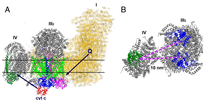
Fig. 4. Scheme of electron flow within the respirasome mediated by cytochrome c and ubiquinol. (A) Side view of the I + III 2 + IV supercomplex. Black arrows point how the ubiquinol and the cytochrome c move between complexes I, III 2 , and IV. (B) Top view of the respirasome fragment consisting of complexes III 2 and IV, seen from the intermembrane space. The distance between cytochrome c binding sites of complexes III 2 and IV is 10 nm. In yellow, the density map of complex I from Yarrowia lipolytica , marked as I; in gray, X-ray structures of bovine complexes III 2 and IV, marked as III 2 and IV correspondingly. Q, ubiquinol; cyt c , cytochrome c . Colors: red, cytochrome c ; dark green, subunit II of complex IV; blue, cytochrome c 1 subunit of complex III 2 ; green, cytochrome b of complex III 2 ; magenta, “Rieske” protein of complex III 2 . Horizontal lines on A indicate the position of the membrane.
