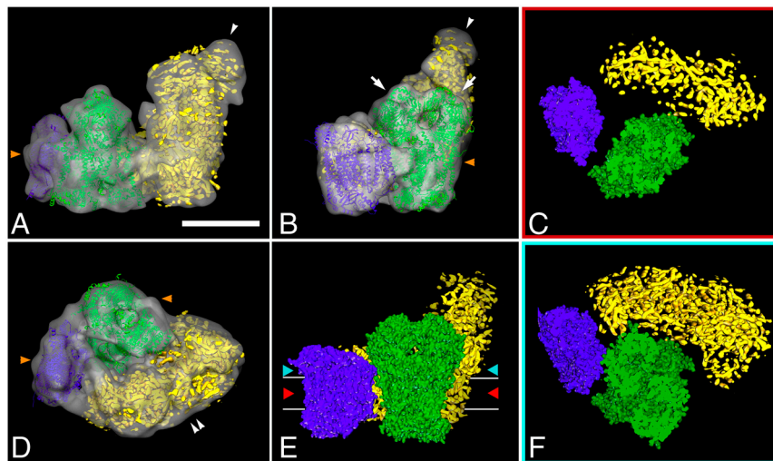
Fig. 3. Fitting of the high- and medium-resolution structures of complexes I, III 2 , and IV to the 3D cryo-EM map of I + III 2 + IV supercomplex: (A) side view, arrowhead points to flavoproteins; (B) side view from the membrane, arrows point to core I and II subunits of complex III 2 , arrowhead to flavoproteins; (C) section through the space-filling model of respirasome on the level of membrane, demonstrating gaps between complexes within the supercomplex; (D) top view from the intermembrane space, double arrowhead points to the bend of complex I in membrane; (E) space-filling model of respirasome seen from the membrane, red and light-blue arrowheads show the level of sections in C and F; (F) section through the space-filling model of respirasome on the level of matrix. In green, X-ray structure of the bovine dimeric complex III; in purple, X-ray structure of bovine monomeric complex IV; in yellow, the density map of complex I from Yarrowia lipolytica . Horizontal lines on E indicate the position of the membrane. Orange arrowheads on A, B, and D point to the position of detergent micelles. (Scale bar: 10 nm.)
